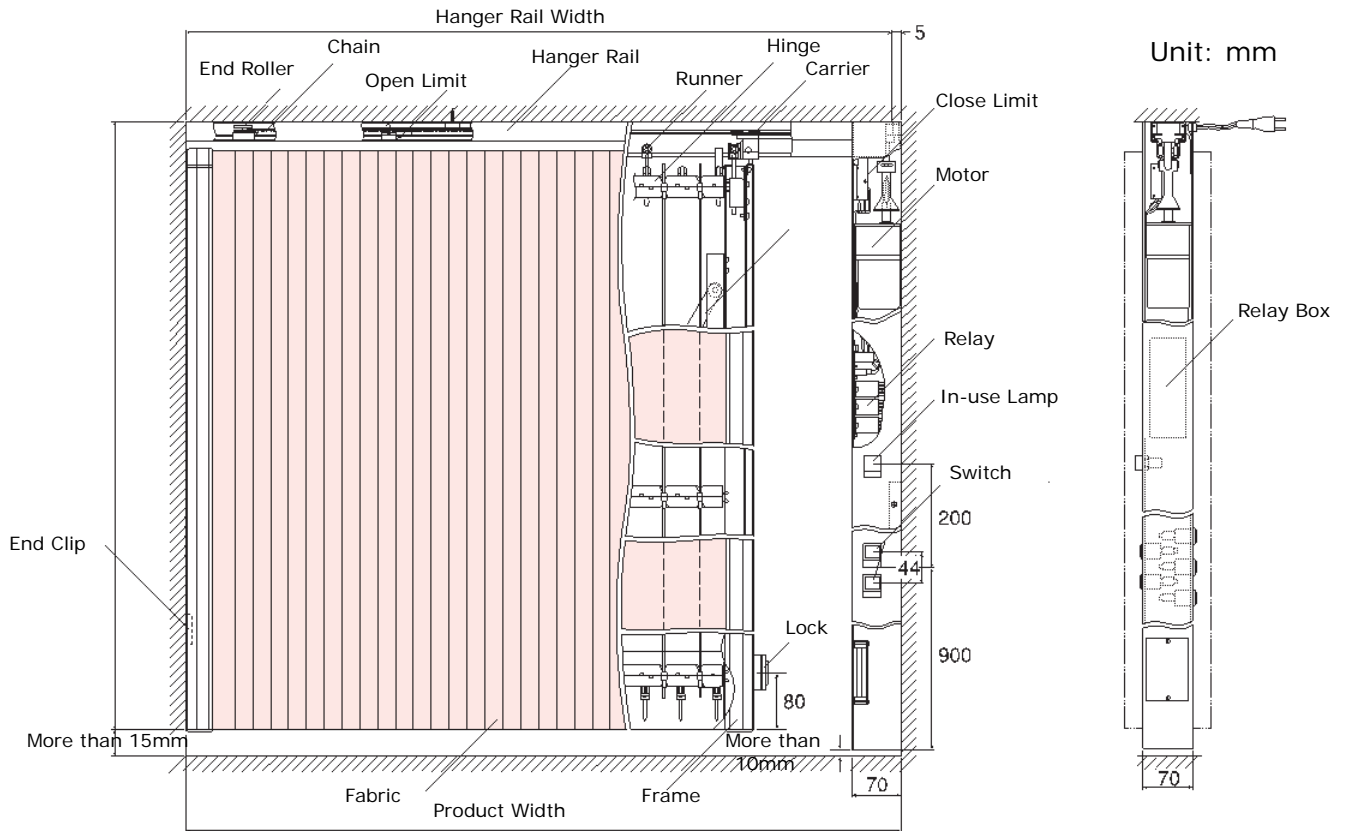
Hanger Rail
