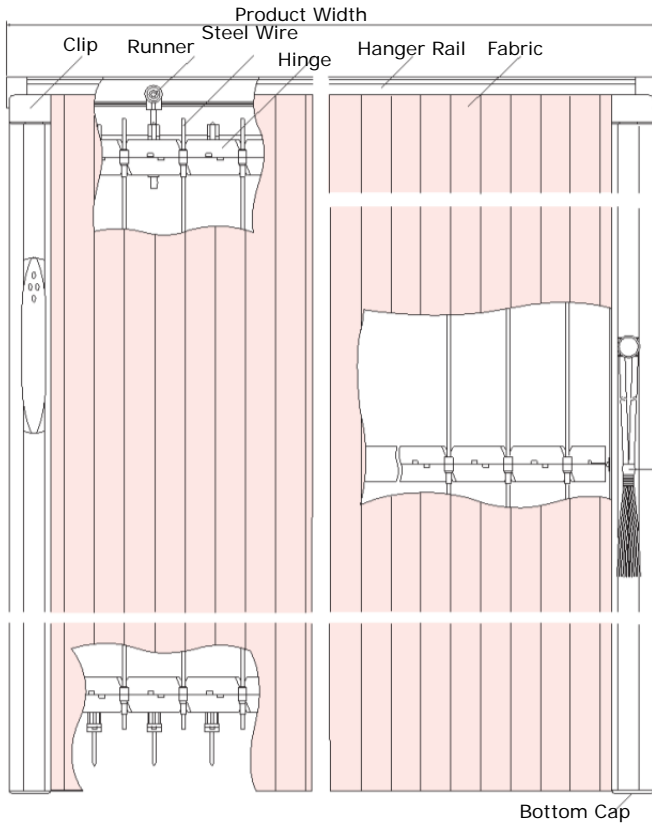
Hanger Rail
