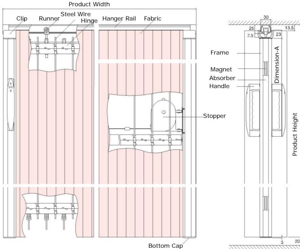
Hanger Rail
