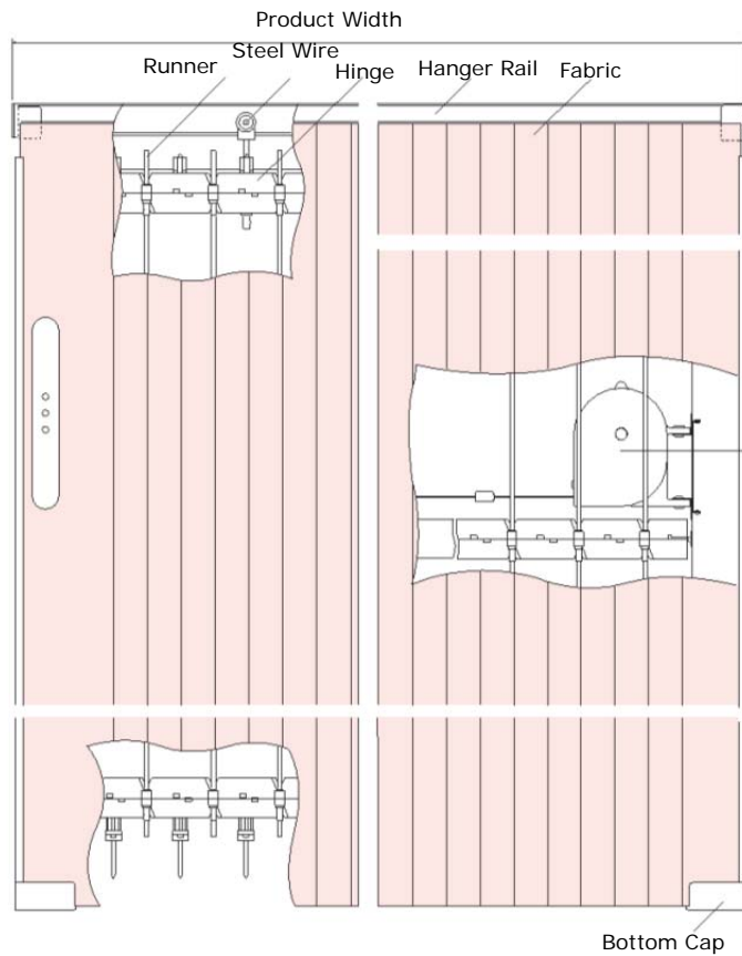
Hanger Rail
