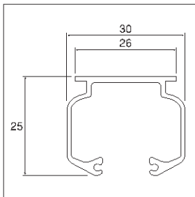
Hanger Rail
