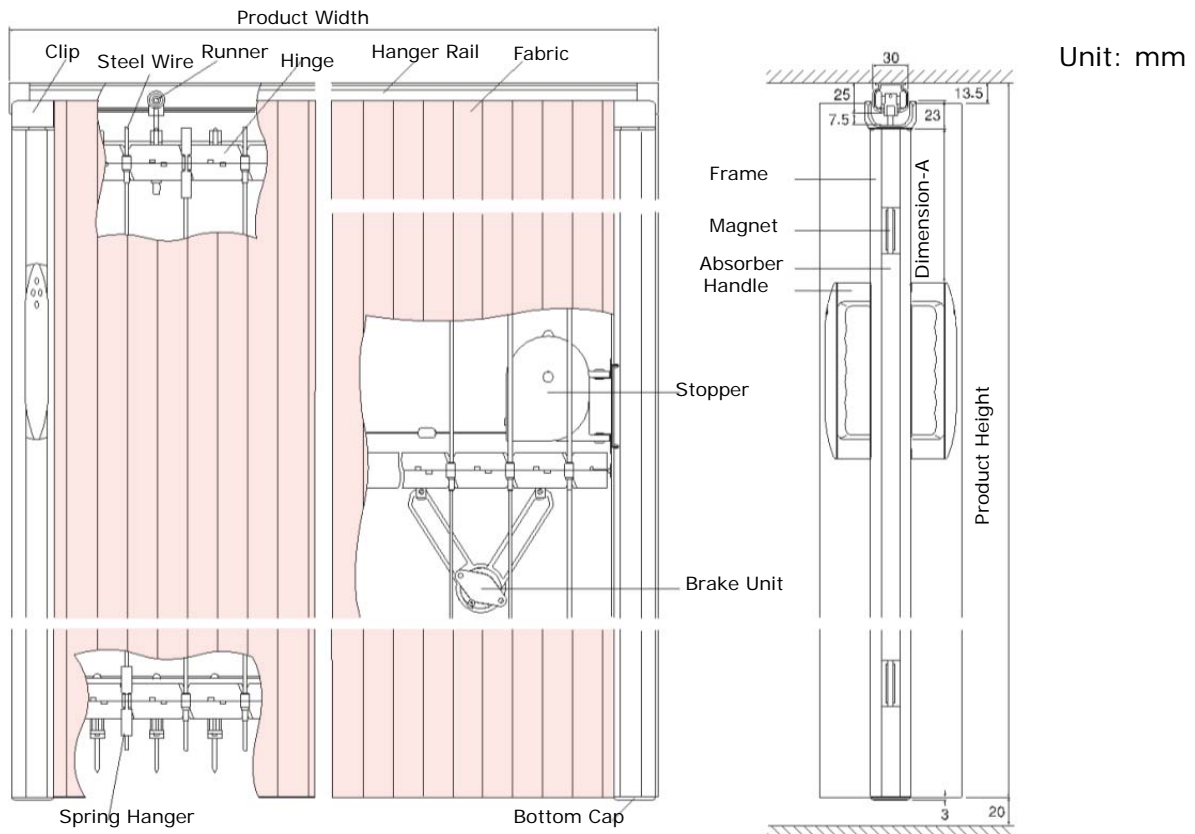
Hanger Rail
