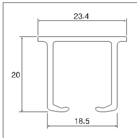
Hanger Rail
